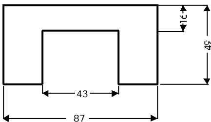
U43 Ⓣ
