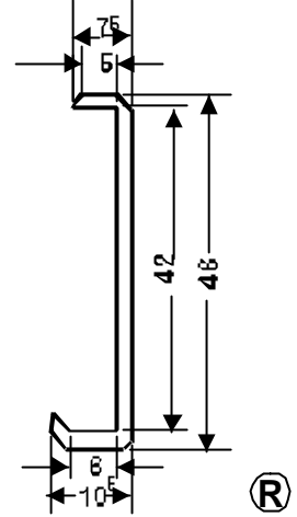
BDA.C42C/TRABA
