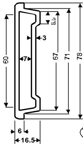
BARANDAC52/115
