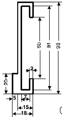
BDA.C82C/REBAJE
