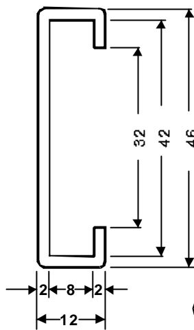
BARANDAC42
