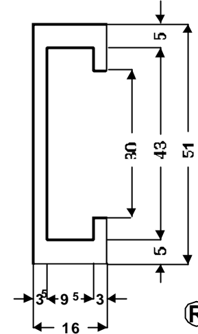
BARANDAC43
